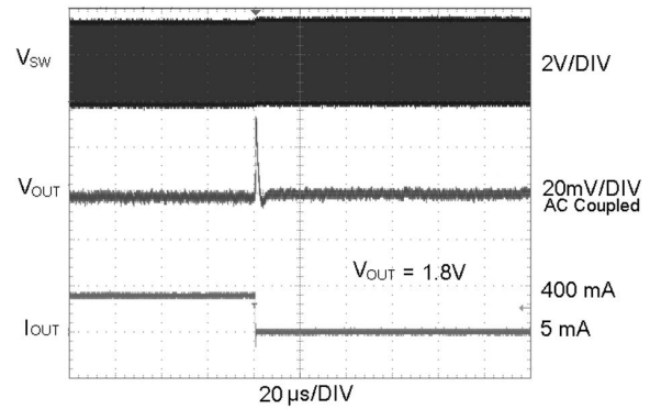
Load Transient Reponse ( V_{OUT} = 1.8V , FPWM Mode)
