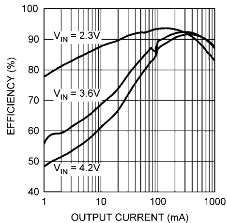
Efficiency vs. Output Current ( V_{OUT} = 1.8V , ECO Mode)
